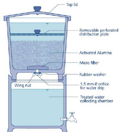
Activated Alumina-based Household Defluoridation (Credit: Lyengar, 2002)
